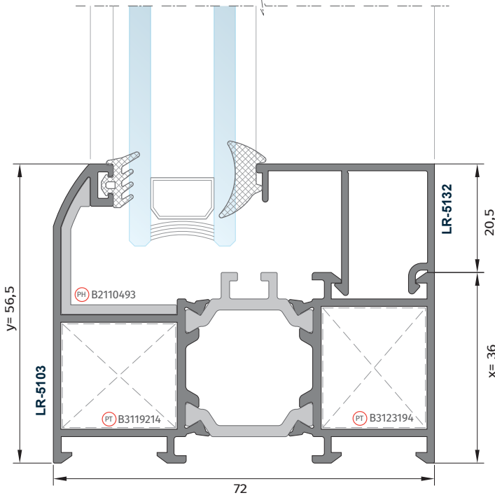
A 101 LR-5103 Kasa Profili LR-5103 Frame Profile
