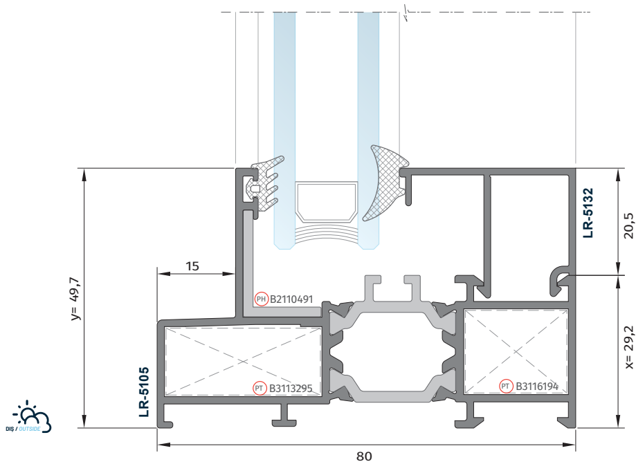
A 101 LR-5105 Kasa Profili LR-5105 Frame Profile
