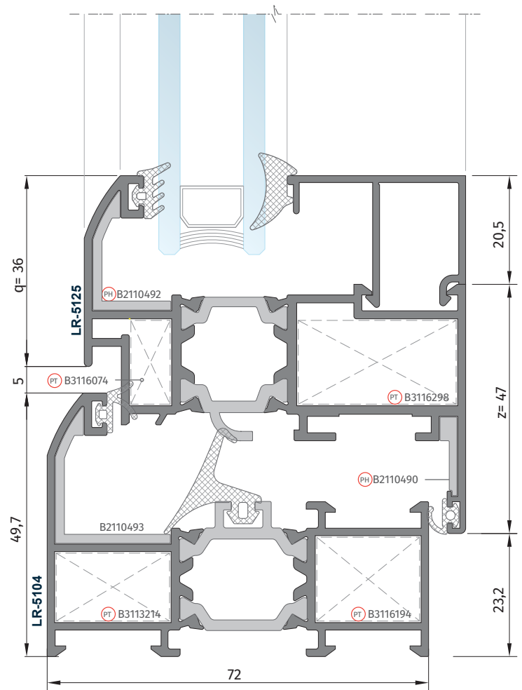
C 103 LR-5125 Kanat Profili (LR-5104 Kasa) LR-5125 Sash Profile (LR-5104)
