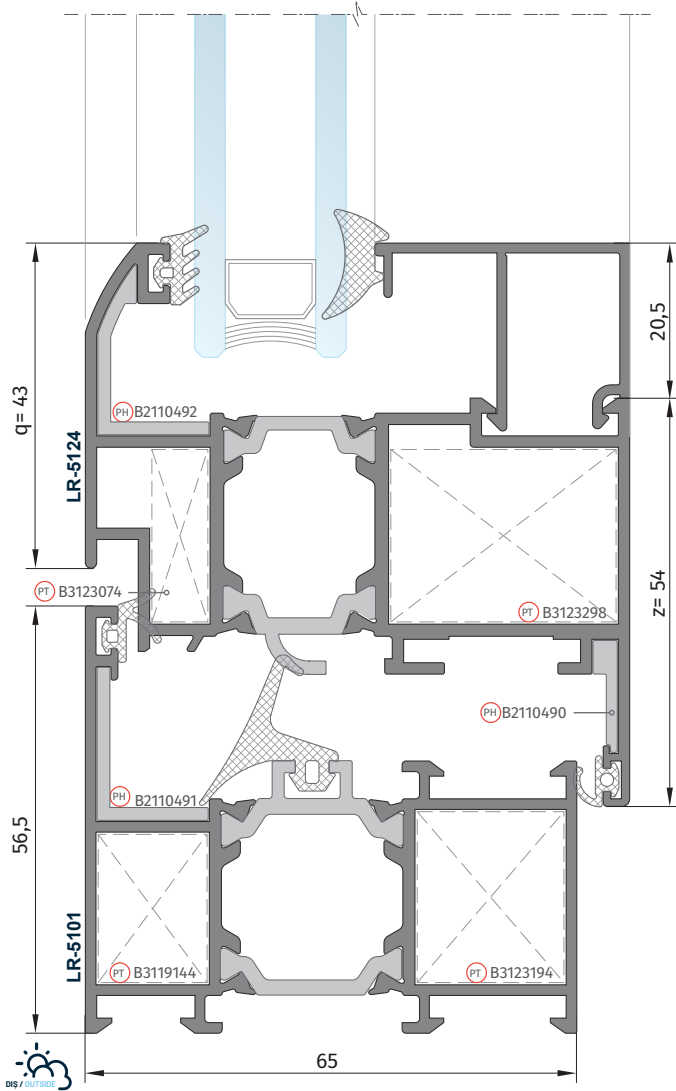
C 103 LR-5124 Kanat Profili LR-5124 Sash Profile
