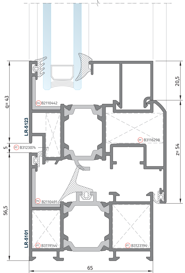
C 103 LR-5123 Kanat Profili LR-5123 Sash Profile
