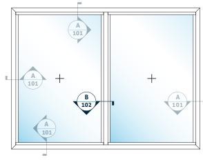
B SABİT 2+ PANEL ÜNİTE 2+ SASH FIXED UNIT
