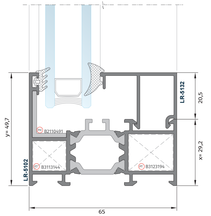
A 101 LR-5102 Kasa Profili LR-5102 Frame Profile
