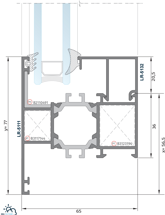
A 101 LR-5111 T Kasa Profili LR-5111 T Frame Profile
