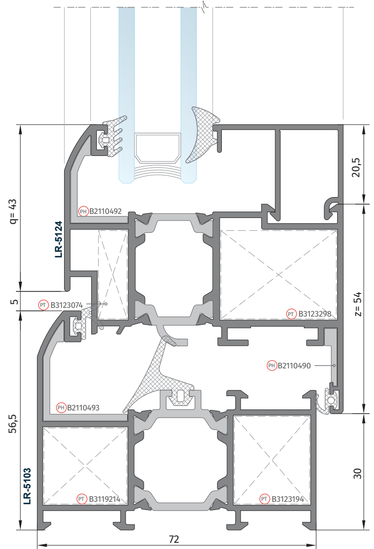
C 103 LR-5124 Kanat Profili (LR-5103 Kasa) LR-5124 Sash Profile (LR-5103)
