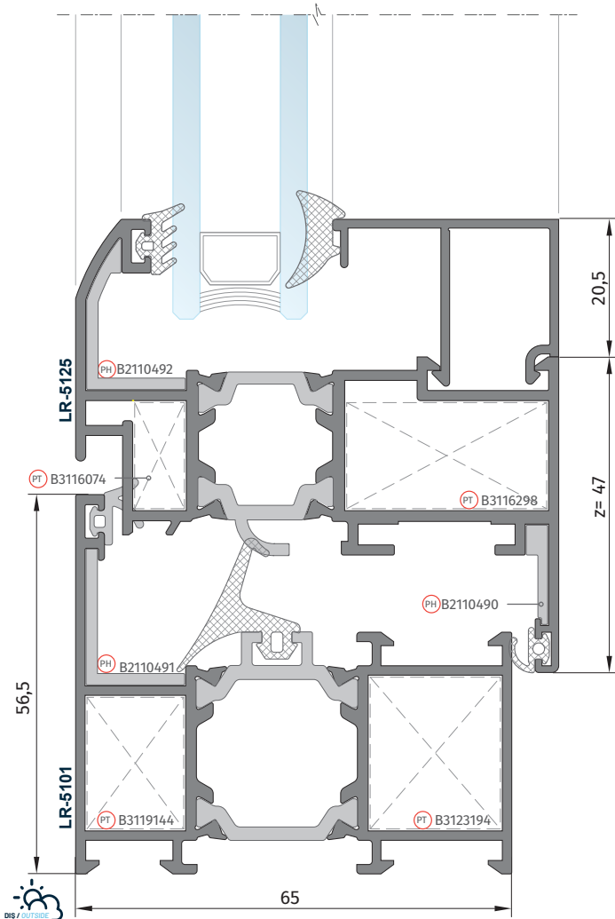
C 103 LR-5125 Kanat Profili LR-5125 Sash Profile
