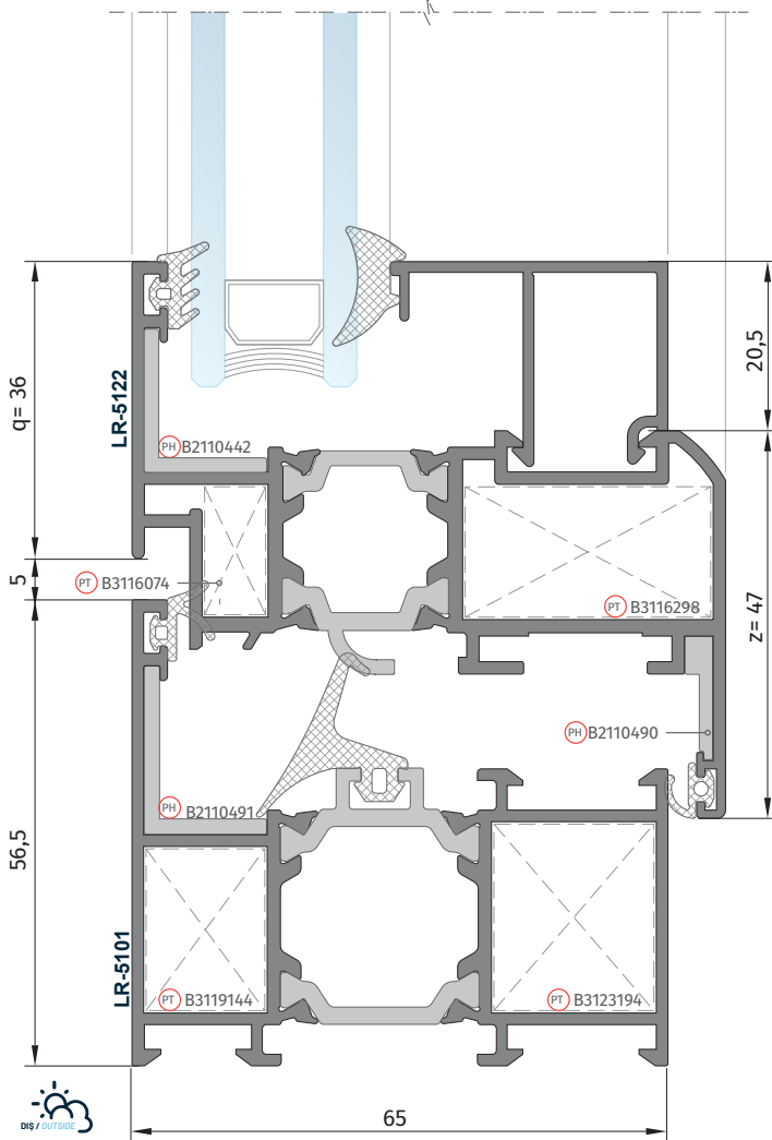
C 103 LR-5122 Kanat Profili LR-5122 Sash Profile
