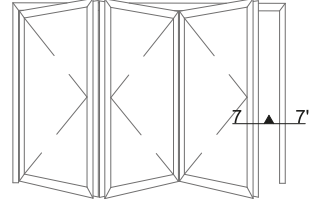
DETAY 7-7' DETAIL 7-7'
