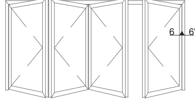
DETAY 6-6' DETAIL 6-6'
