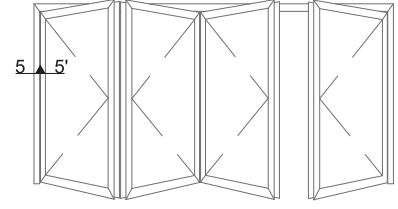
DETAY 5-5' DETAY 5-5'
