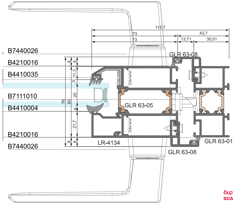
DETAY 7-7' DETAIL 7-7'
