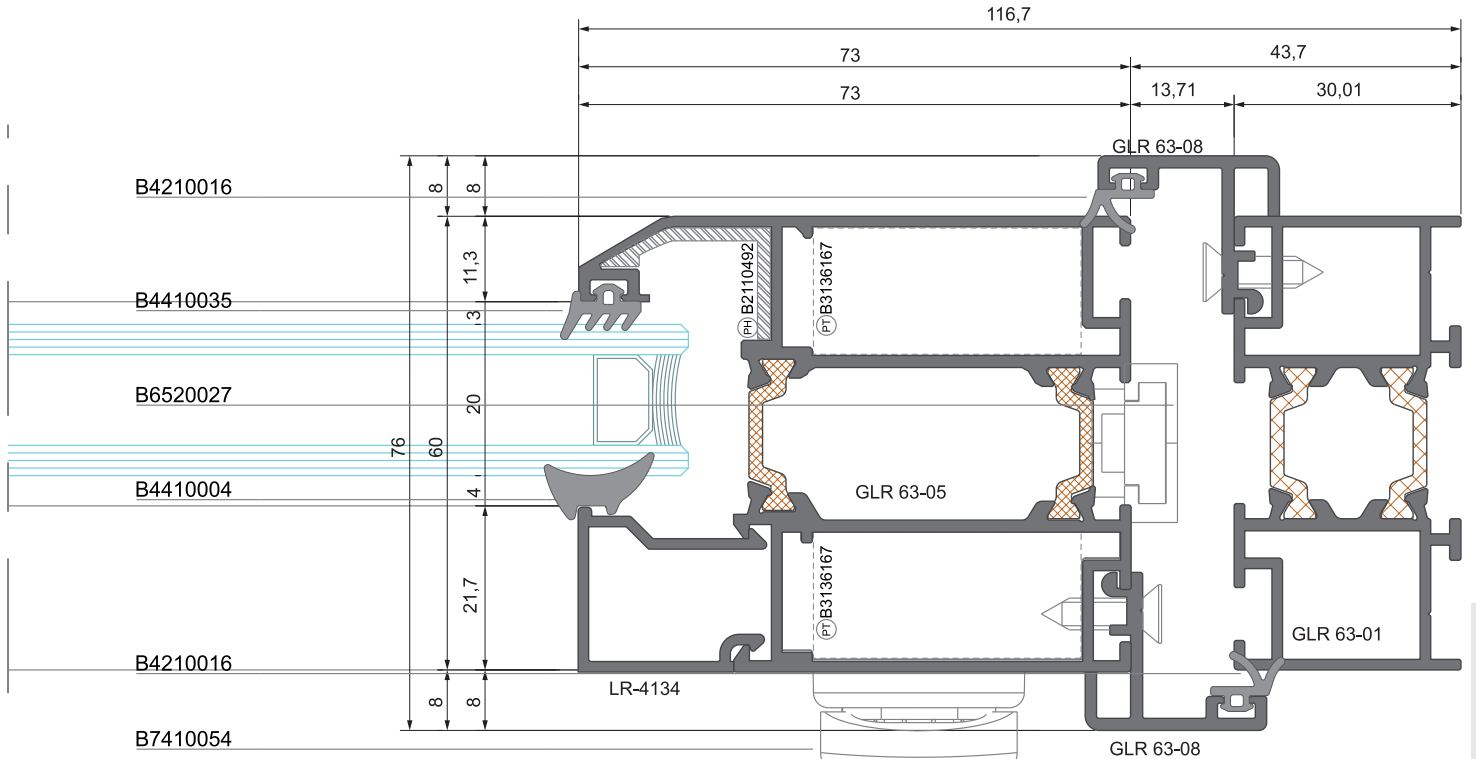
DETAY 7-7' DETAIL 7-7'
