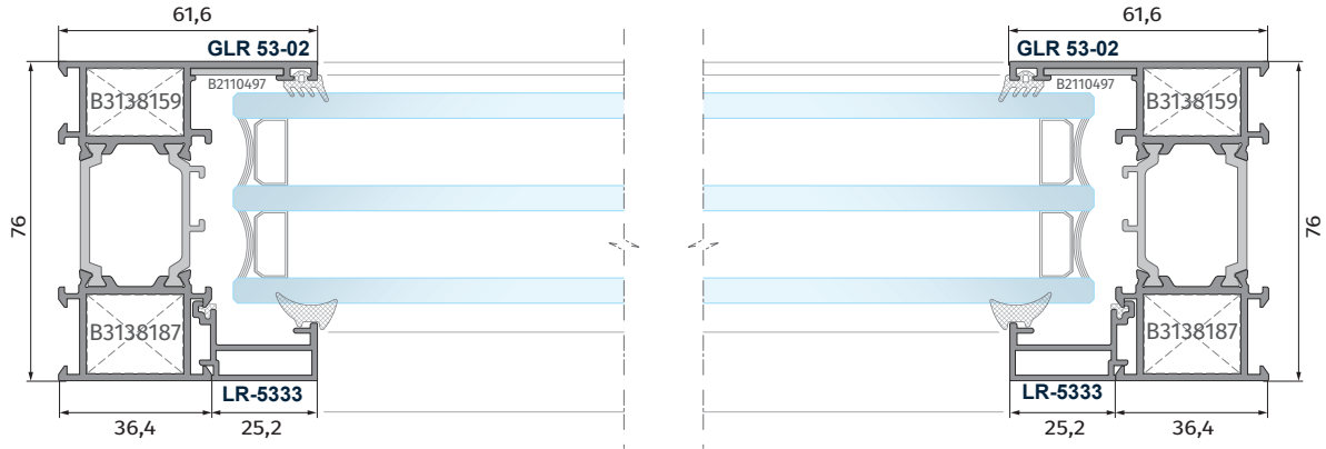
B İnce Kasa Sabit Panel Detayı 102 Thin Fixed Panel Detail
