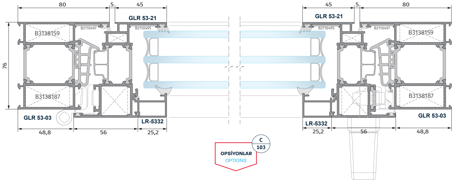
C Açılır Panel Detay 103 Opening Panel Detail
