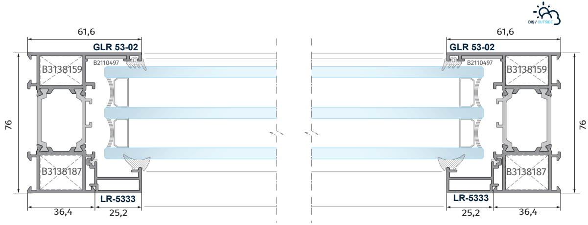
B 102 İnce Kasa Sabit Panel Detay Thin Fixed Panel Detail
