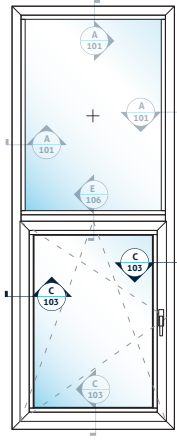
C Açılır Panel Detay 103 Opening Panel Detail
