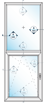
B İnce Kasa Sabit Panel Detayı 102 Thin Fixed Panel Detail
