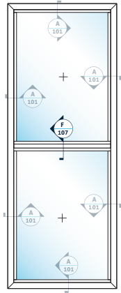
H ORTAKAYIT BİRLEŞİM SABİT+SABİT TRANSOM CONNECTION FIX+FIX
