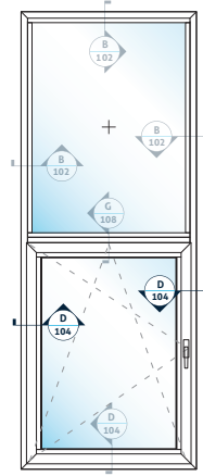
D Açılır Panel Detay 104 Opening Panel Detail
