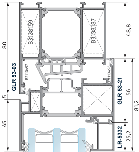
C Açılır Panel Detay 103 Opening Panel Detail
