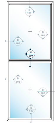
J İNCE KASA BİRLEŞİM SABİT+SABİT THIN SASH CONNECTION FIX + FIX
